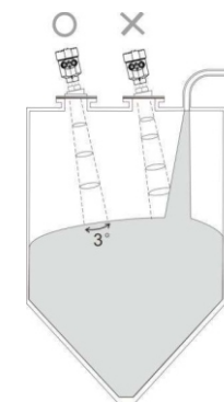
Antenna beam avoids the feed inlet
