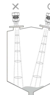
The conical tank shall ensure that the beam is directed at the tank bottom as far as possible
