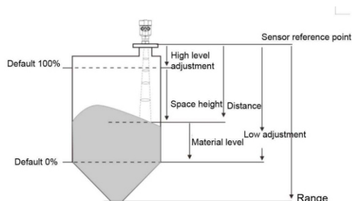
Low position adjustment editing interface and definition
