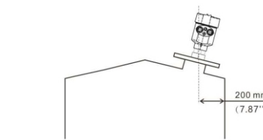
The installation shall be at least 20cm away from the vessel wall
