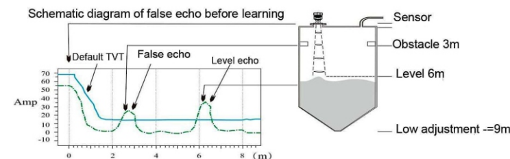
Schematic diagram of false echo before learning
