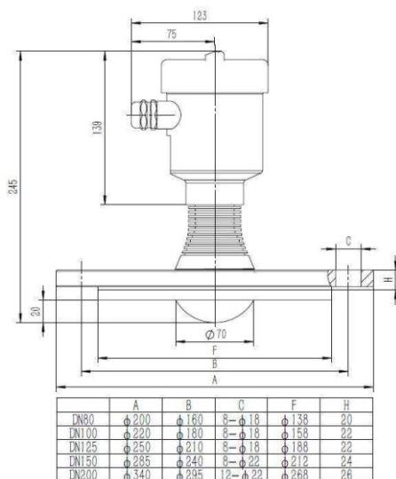
Schematic Diagram of High Temperature and High Pressure Structure Dimension of Anticorrosive Flange(unit: mm)
